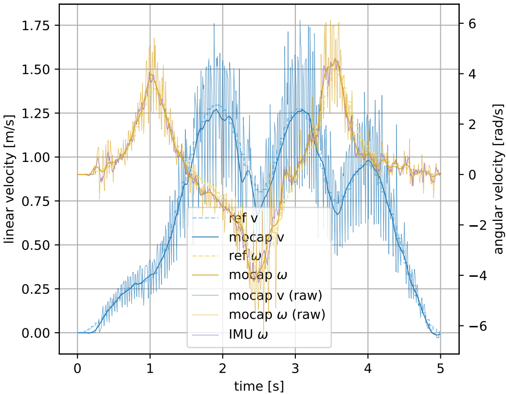
Velocity
