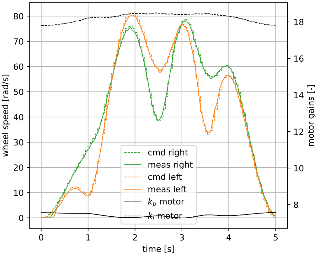
Wheel Speeds
